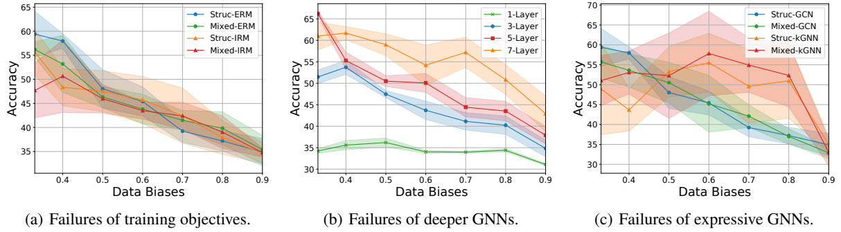
Figure 7. Failure of existing methods on SPMotif with FIIF attribute shifts and graph size shifts.
