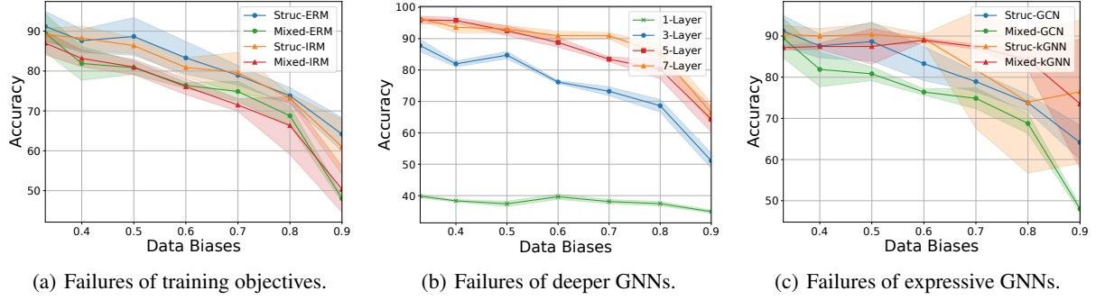
Figure 6. Failure of existing methods on SPMotif with FIIF attribute shifts.
