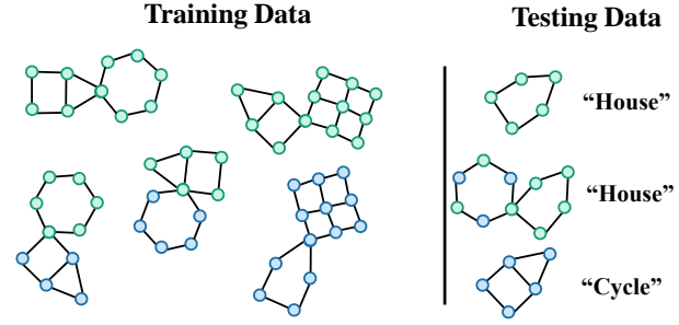
Figure 5. Failure cases for existing methods. GNNs are required to classify whether the graph contains a “house” or “cycle” motif, where the colors represent node features. However, distribution shifts in the training exists at both structure level (From left to right: “house” mostly co-occur with a hexagon), attribute level (From upper to lower: graphs nodes are mostly green colored if they contain “house”, or blue colored if they contain “cycle”), and graph sizes, making GNNs hard to capture the invariance. ERM can fail for leveraging the shortcuts and predict graphs that have a hexagon or have mostly green nodes as “house”. IRM can fail when testing data are not sufficiently supported by the training data.
